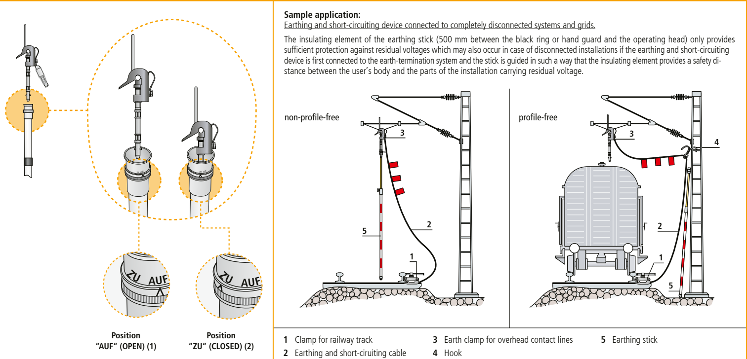
Fig. 6 Example of an aluminium cone coupling connected to energised parts
