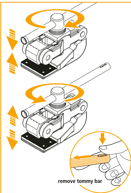
Fig. 3 Railway track connection clamp with tommy bar
