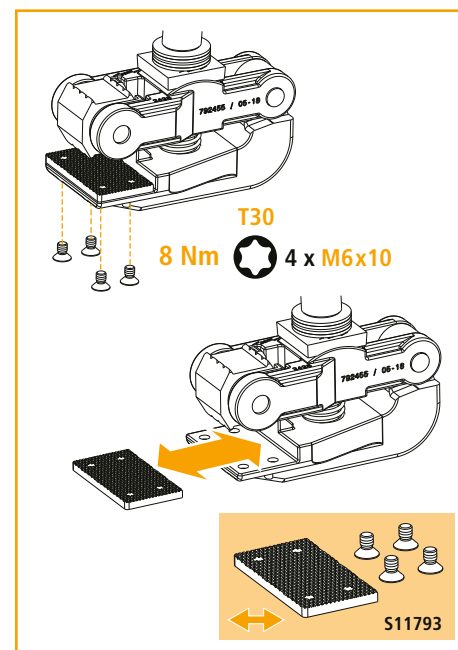
Fig. 5 Exchange of contact plate
