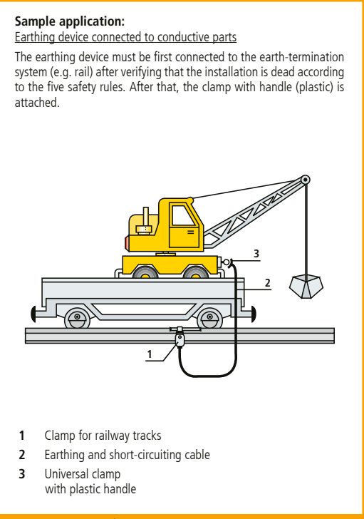
Fig. 7 Example of an earthing and short-circuiting connected to de-energised parts
