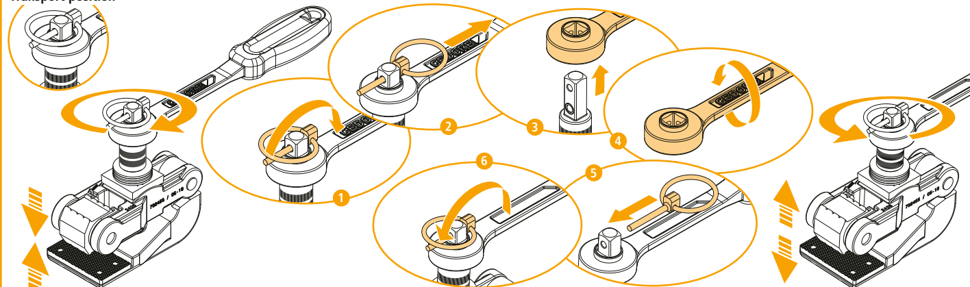
Fig. 2 Railway track connection clamp with ratchet
