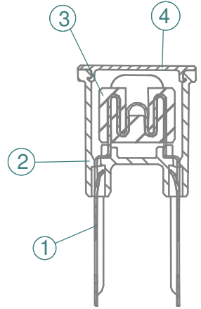
Cross section scale 1:1
