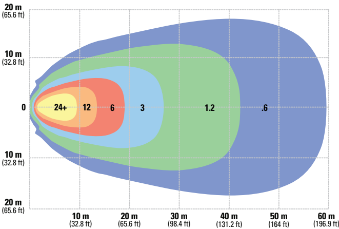
1800 Lumen Near Pattern
