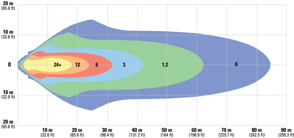
1800 Lumen Far Pattern
